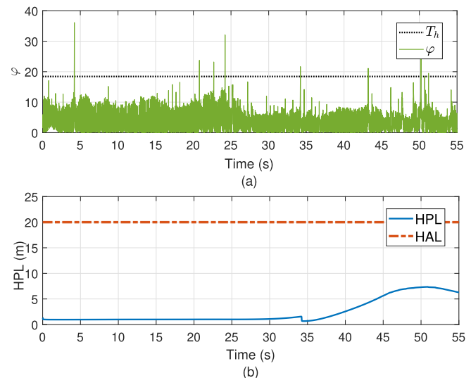
Fig. 19. Environment 2 experimental results: resulting fault detection test and exclusion; (a) the fault detection test which compares the test statistic \phi against the detection threshold T_h , (b) The HPL and HAL over the course of the experiment.
