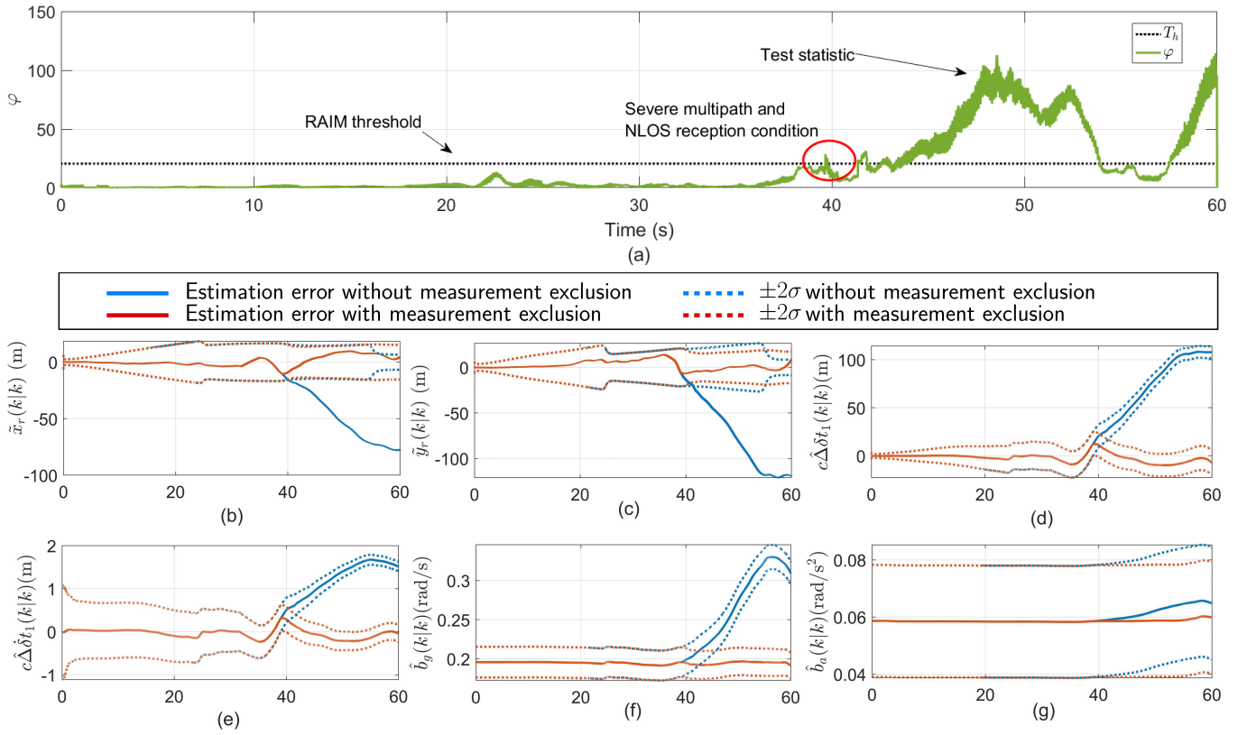
Fig. 14. Environment 1 experimental results: resulting fault detection test and exclusion; (a) the fault detection test which compares the test statistic \varphi against the detection threshold T_h , (b)–(c) the resulting position estimation errors and corresponding \pm 2\sigma bounds with and without using the proposed fault exclusion, (d)–(e) the estimated receiver’s clock error states, and (f)–(g) The resulting estimation and corresponding variances for IMU gyroscope and accelerometer biases.
