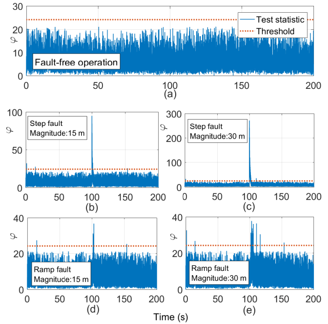
Fig. 10. The resulting test statistic for the faults with ramp and step profile. As can be seen, the framework has a similar performance to detect faults with a step and ramp profiles.
