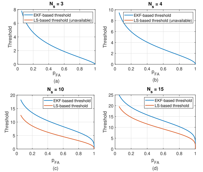
Fig. 6. The threshold for LS-based and EKF-based test statistics for N_s = 3, 4, 10, and 15 transmitters. As can be seen, the LS-based threshold for N_s = 3 and N_s = 4 is unavailable due to not having sufficient degrees of freedom.
